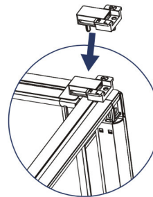
5 Mega-Hanging connector
