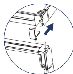
5 Mega-Hanging connector
