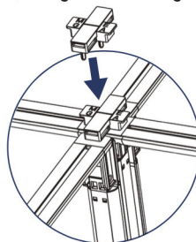
6 Mega-180° Top/Bottom connector
