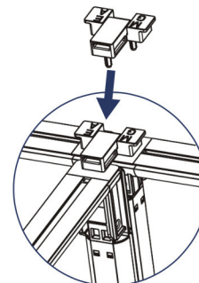
5 Mega-Hanging connector
