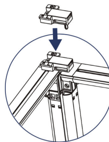
4 Mega-Cross fitting
